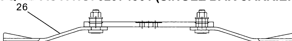
SQ HD ASY. NO. 02974861 (SINGLE BAR CARRIER)
